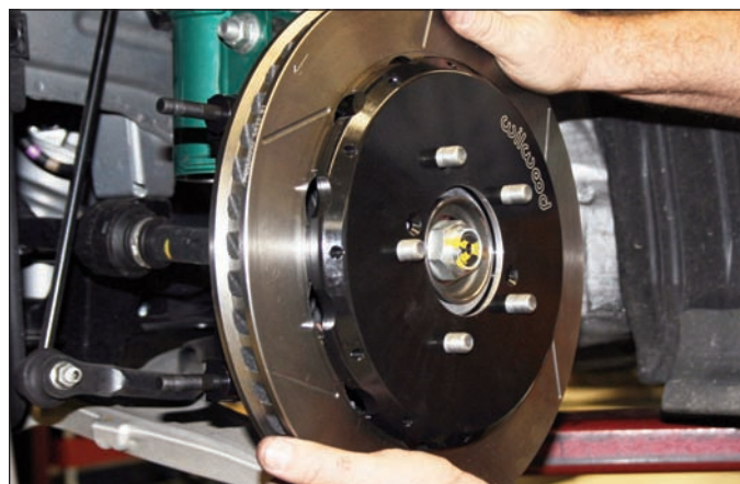
Sequence 18: Install the hat/rotor assembly over the studs on the hub assembly. NOTE: The hat/rotor must fit flush against the axle hub flange or excessive rotor run out may result.
