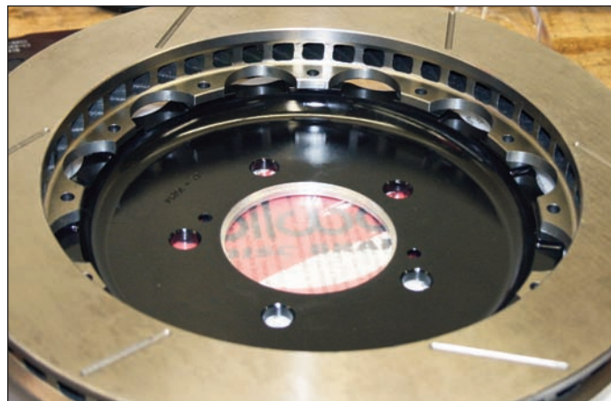
Sequence 16: The hat needs to be bolted to the rotor. Orient the rotor over the hat in the configuration shown above.
